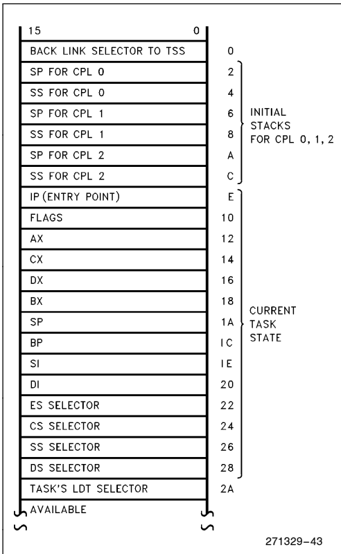
Figure 6-16. 80286 TSS
