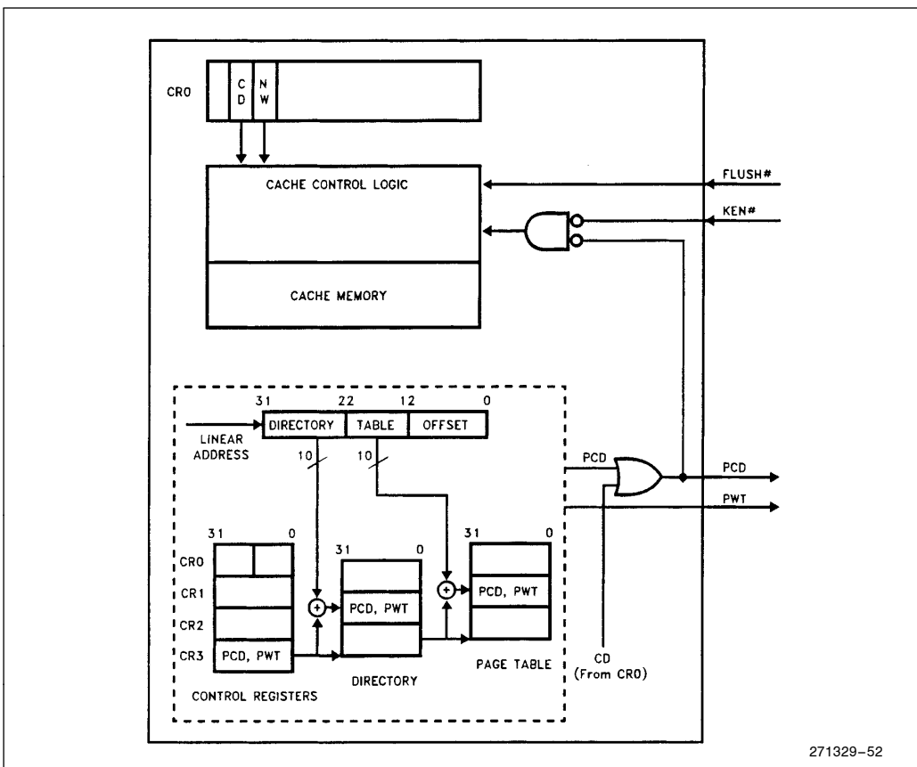
Figure 7-3. Page Cacheability
