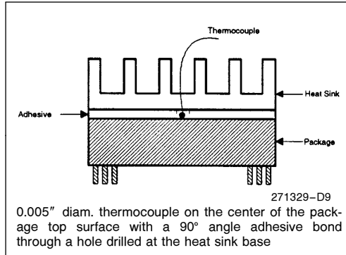
Figure 16-3. Case Temperature Measurement with Heat Sink
