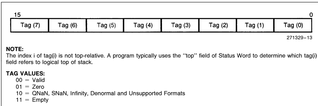
Figure 4-9. Floating Point Tag Word
