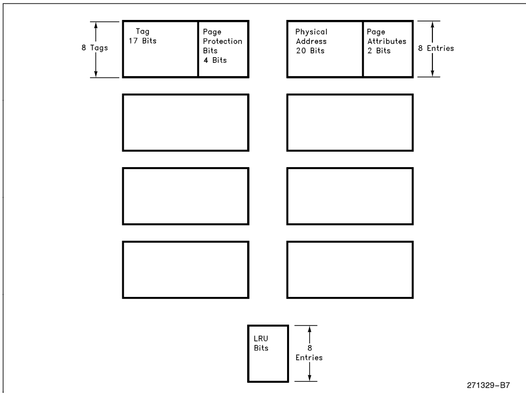
Figure 11-5. TLB Organization
