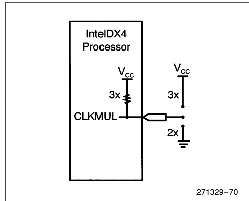
Figure 9-3. Voltage Detect (VOLDET) Sense Pin
