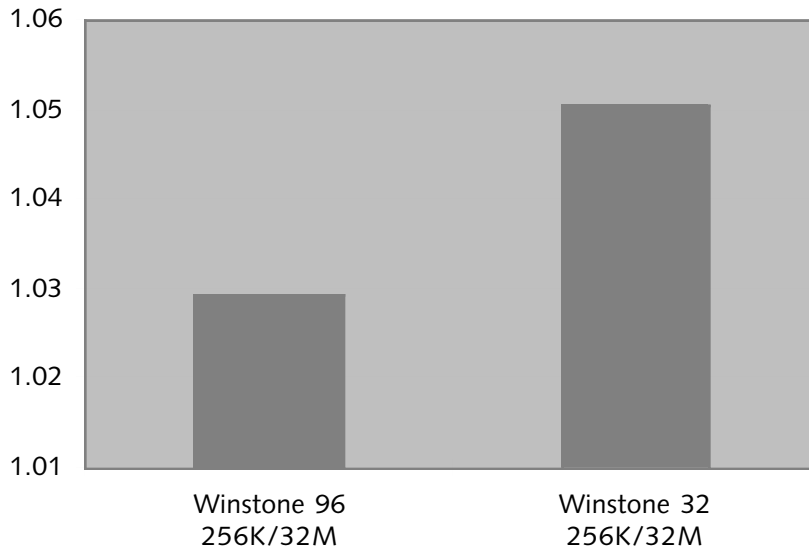
Figure 4. MDR Labs results for the performance of the 6x86 at 150 MHz, relative to the performance of a Pentium-200 in a comparable system configuration. Both systems have 256K cache and 32M DRAM.
