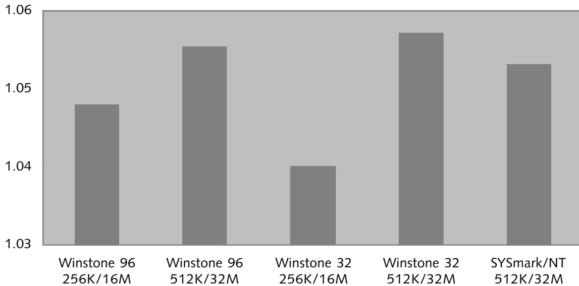
Figure 2. MDR Labs results for the performance of the 6x86 at 120 MHz, relative to the performance of a Pentium-150 in an identical system configuration.
