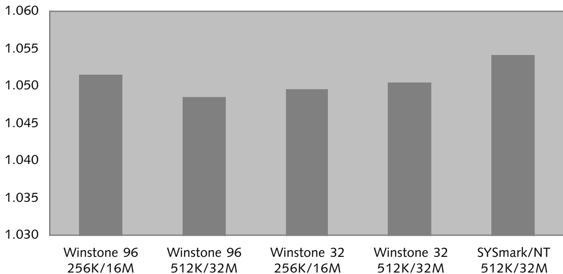
Figure 3. MDR Labs results for the performance of the 6x86 at 133 MHz, relative to the performance of a Pentium-166 in an identical system configuration.
