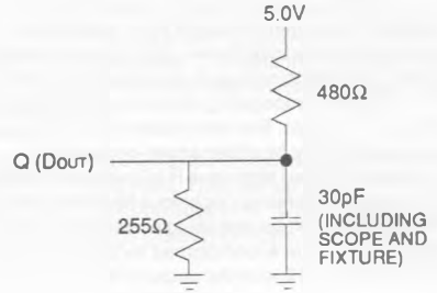
FIGURE 1. OUTPUT LOAD
