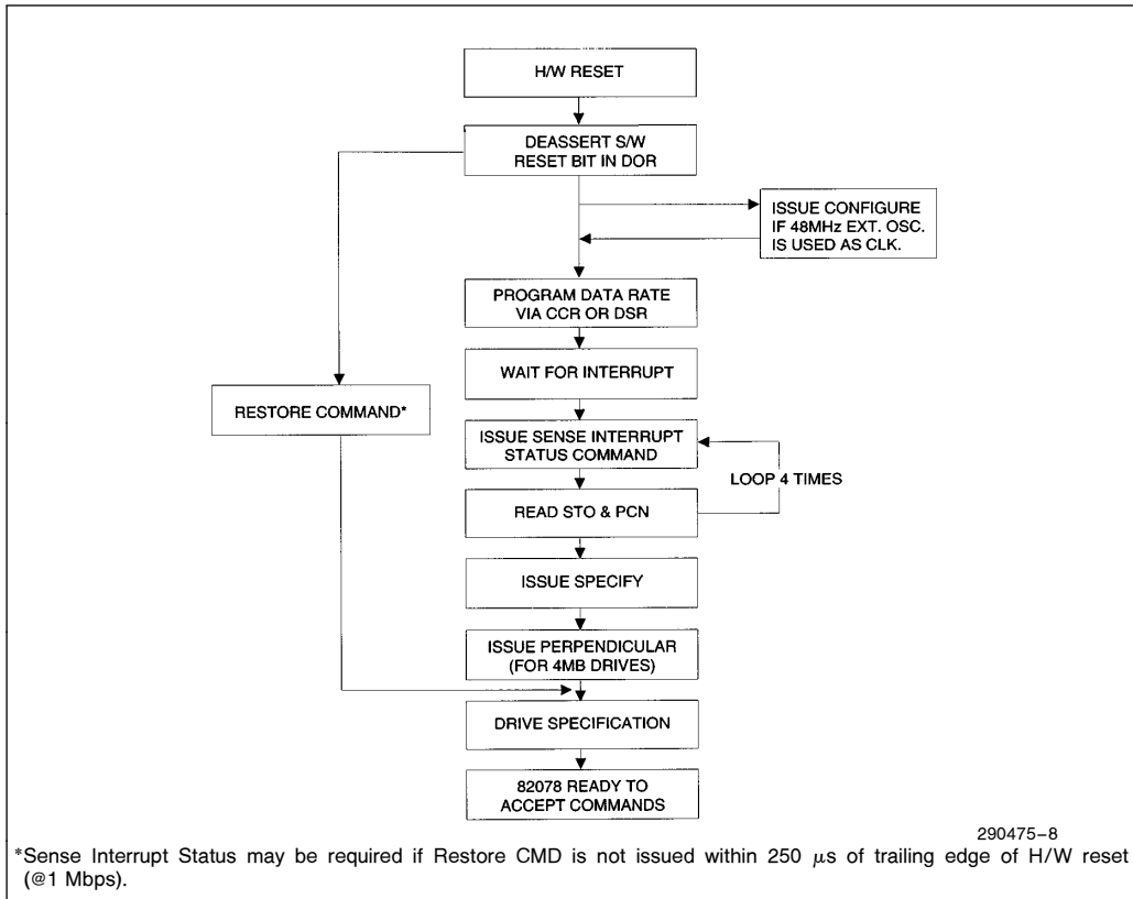
Figure 9-3. Initialization Flowchart
