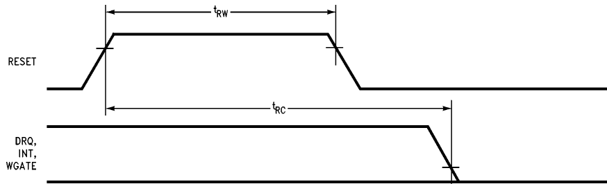
FIGURE 6-5. Reset Timing
