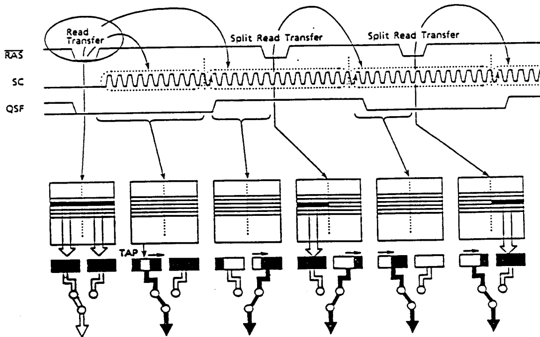
Figure 21. Example of Consecutive Read Transfer Operations
