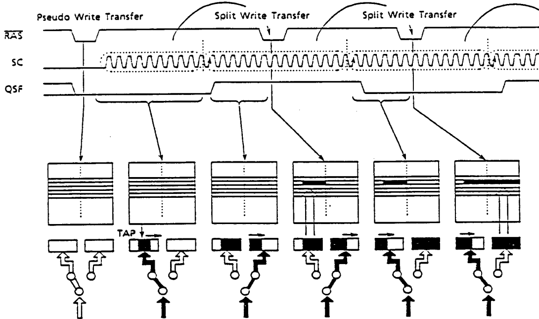
Figure 24. Example of Consecutive Write Transfer Operations
