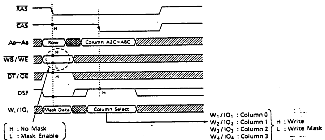
Figure 7. Block Write Timing
