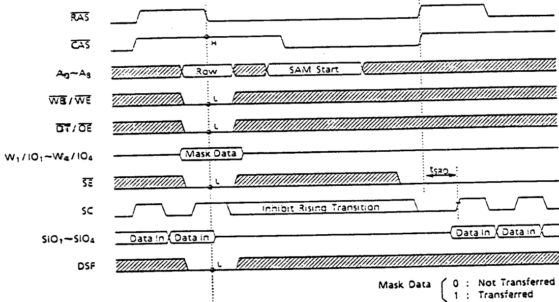
Figure 15. Write Transfer Timing
