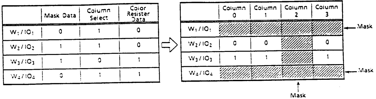
Figure 8. Example of Block Write Operation
