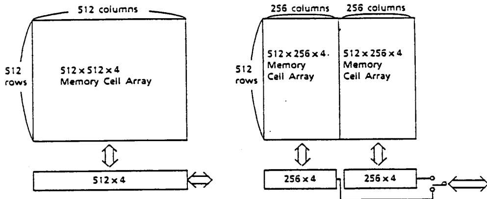
(b) Split Transfer
