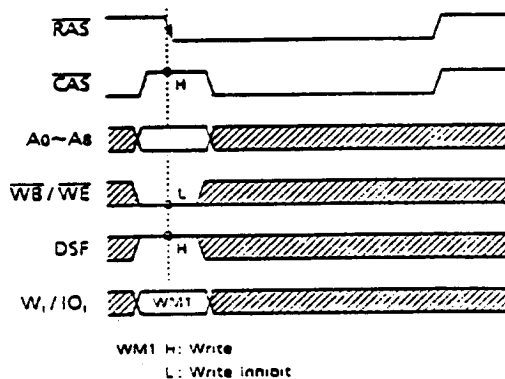
Figure 4. Flash Write Timing
