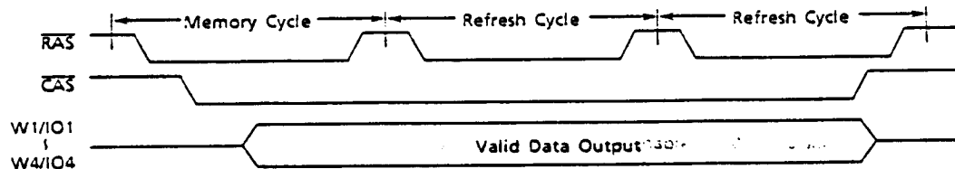
Figure 1. Hidden Refresh Cycle
