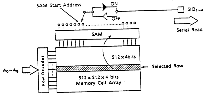
Figure 12. Block Diagram for Read Transfer Operation
