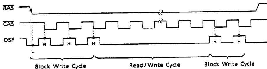
Figure 10. Fast Page Mode Block Write Cycle
