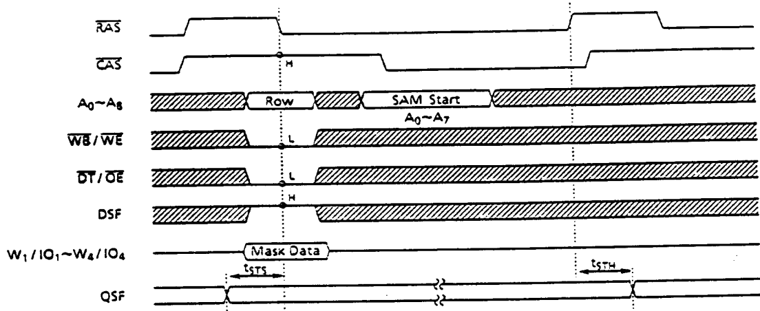
Figure 23. Timing Diagram for Split Write Transfer
