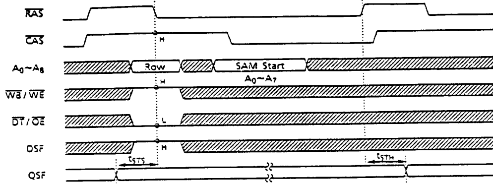
Figure 20. Timing Diagram for Split Read transfer
