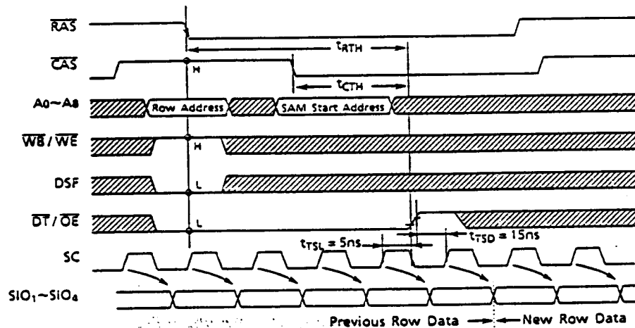
Figure 14. Real Time Read Transfer
