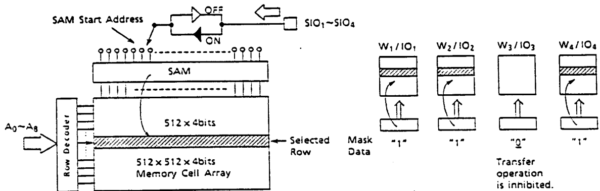
Figure 16. Block Diagram for Write Transfer Operation
