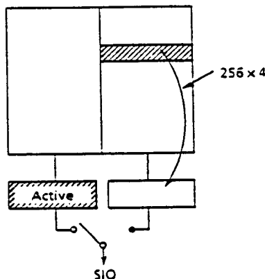
Figure 19. Block Diagram for Split Read Transfer
