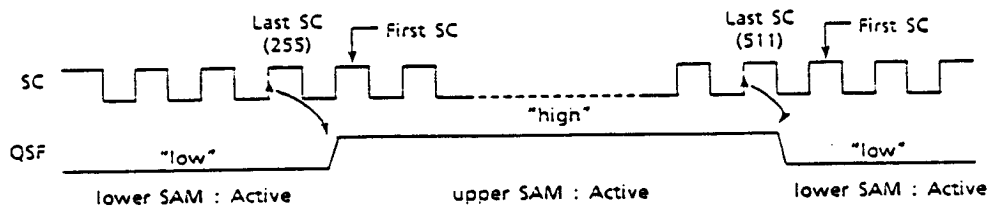
Figure 18. QSF Output State During Split Register Mode
