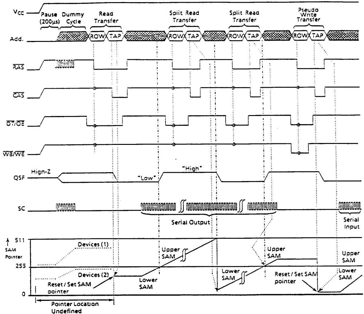
Figure 25. Example of Split SAM Register Operation Sequence
