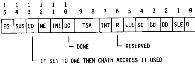
Figure 64. SCB End Status Word 1
