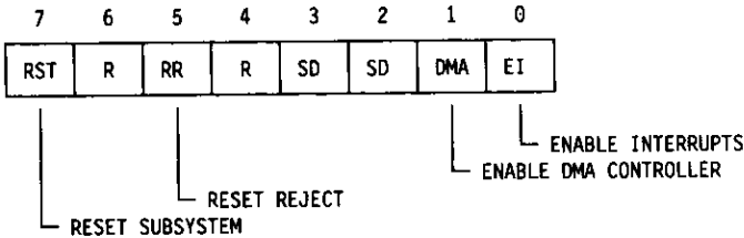
Figure 66. SCB Subsystem Control Register
