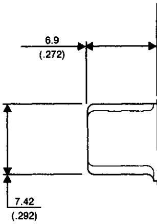
Figure 71. 60-Pin External Connector, Side View
