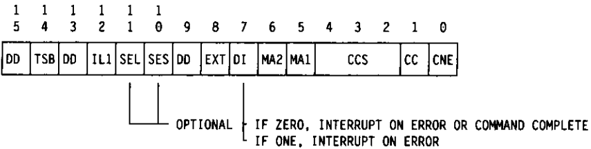
Figure 63. SCB Enable Word 1
