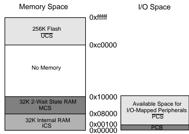
Figure 2. 64 Kbyte RAM Configuration
