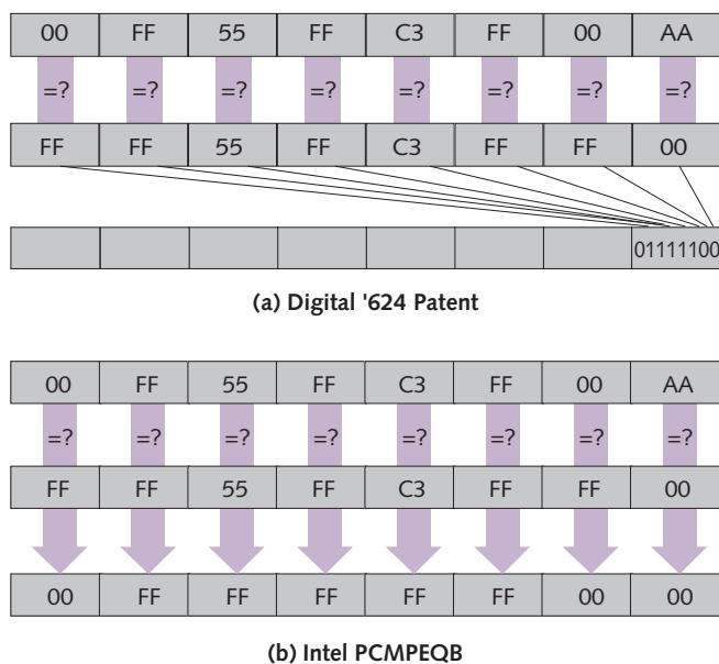
Figure 1. (a) Digital's '624 patent describes a parallel comparison operation. (b) Intel's PCMPQB instruction has a similar function but encodes the result in bytes, not bits.
