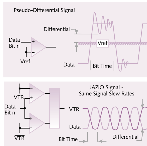
Figure 5. JAZiO differential signaling is compared with pseudo-differential signaling. Noise margin is increased and higher data throughput is achieved with the same slew rate. The noise margin can be traded off for lower signal levels, which can also help to lower signal slew rates.
