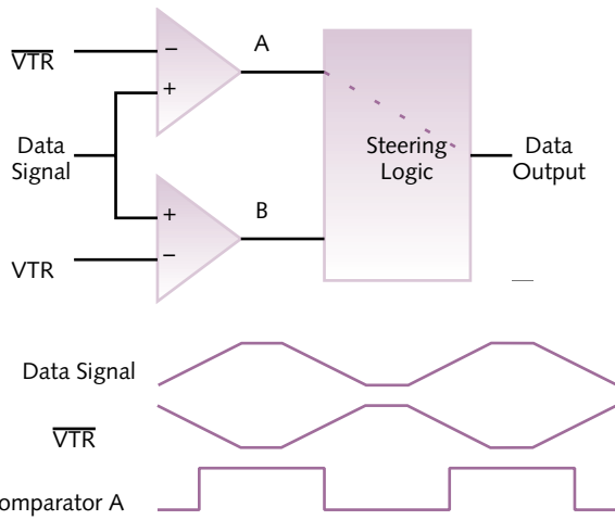
Figure 2. The input data signal is compared against both VTR and its complement. The switching logic selects the correct comparator. An example data waveform is shown against the VTR# signal, forming a differential signal output from comparator A.
