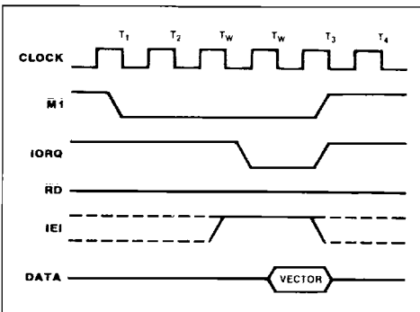
Figure 5c : Interrupt Acknowledge Cycle.
